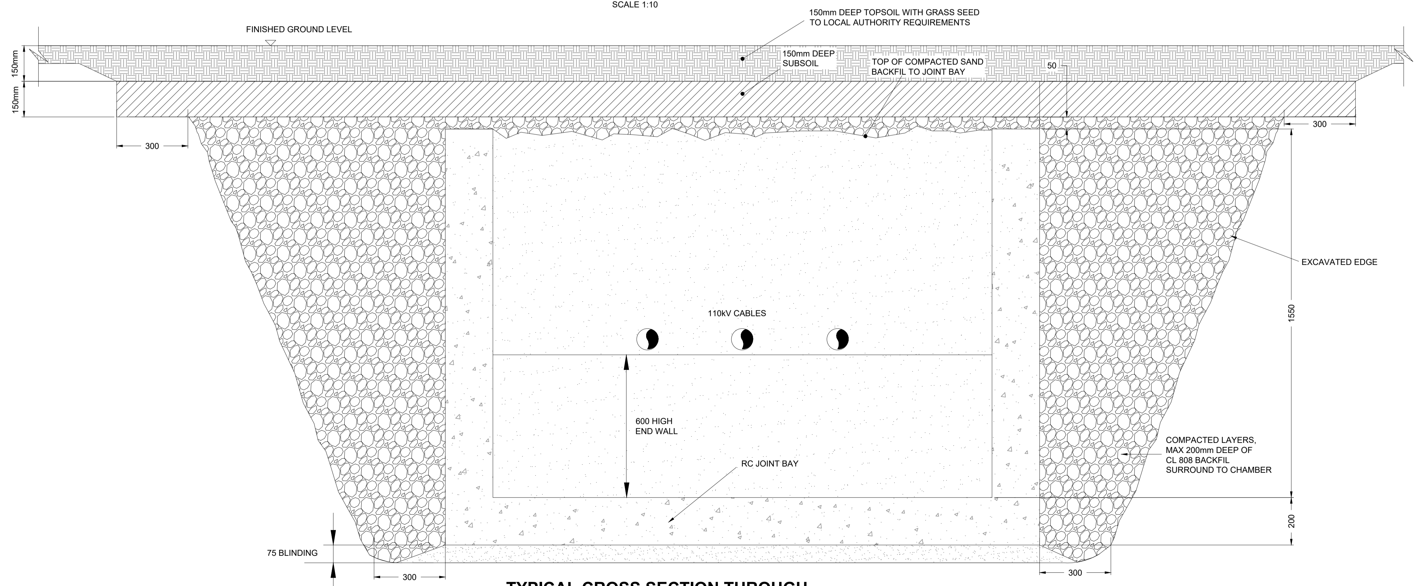
TYPICAL CROSS SECTION THROUGH JOINT BAY UNDER GRASS SCALE 1:10
