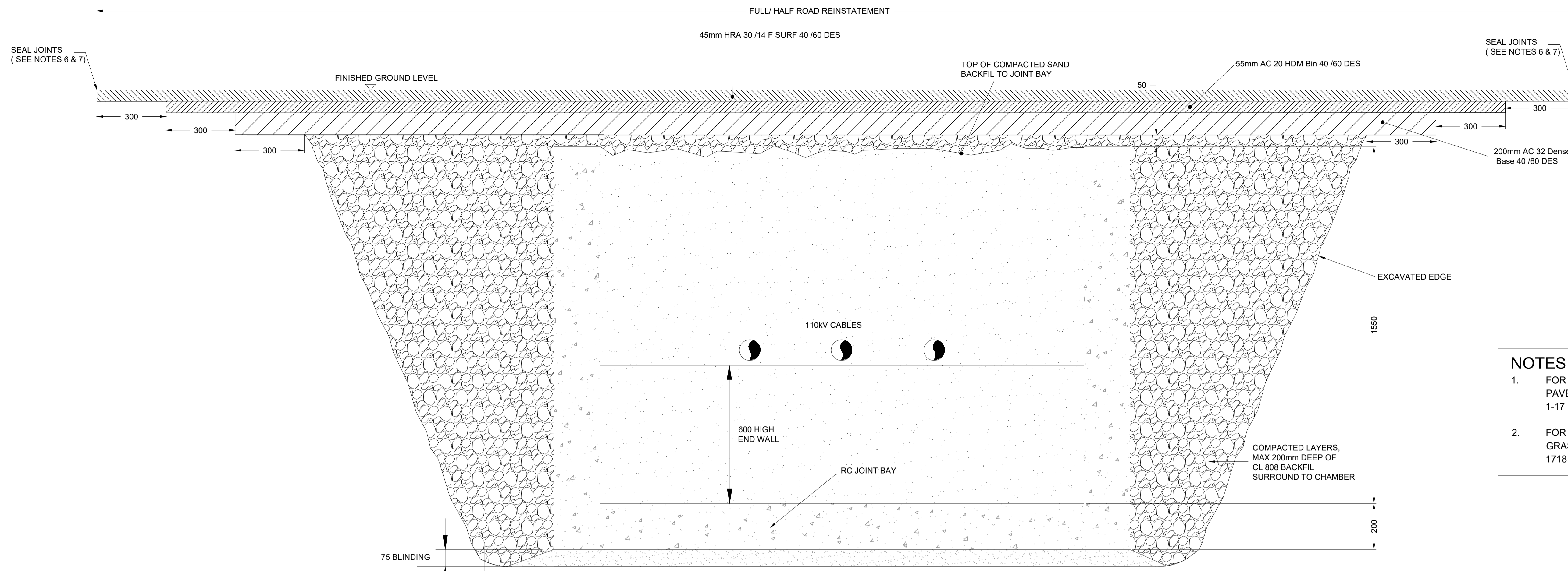
TYPICAL CROSS SECTION THROUGH JOINT BAY UNDER ROAD SCALE 1:10
